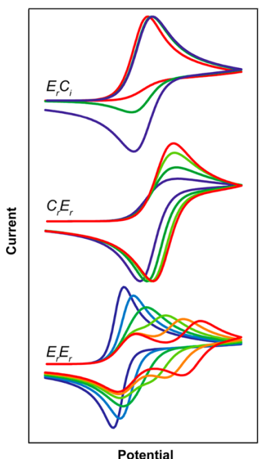
Figure 1. Examples of voltammograms modeled using DigiElch simulation software for three common mechanisms. E r C i mechanism: increasing the scan rate (from u = 0.1 (red) to 1 (green) to 10 \text{ V s}^{-1} (blue)) restores reversibility (rate constant for the C i step k = 5 \text{ s}^{-1} ).
